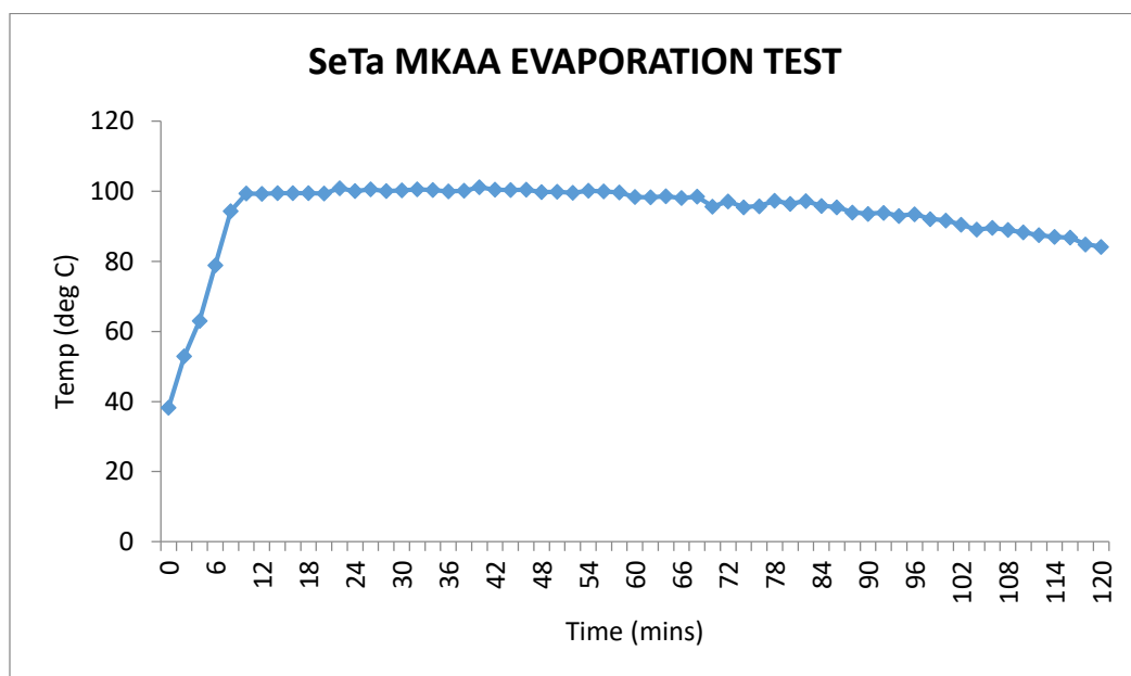
Figure 4.1: Evaporation Test
